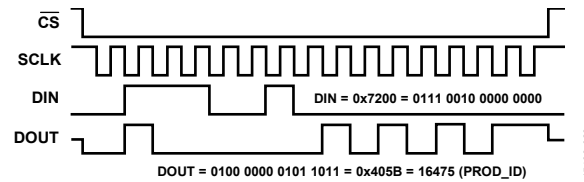
Figure 26. SPI Signal Pattern, Repeating Read of the PROD_ID Register
