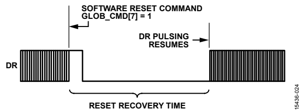
Figure 22. Data Ready Response During Reset (Register GLOB_CMD, Bit 7 = 1) Recovery
