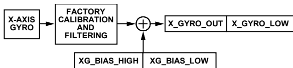
Figure 38. User Calibration Signal Path, Gyroscopes
