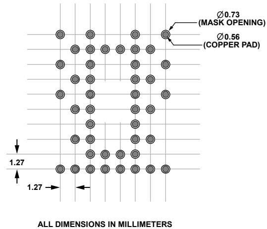
Figure 45. Recommend PCB Pattern, Solder Mask Defined Pads
