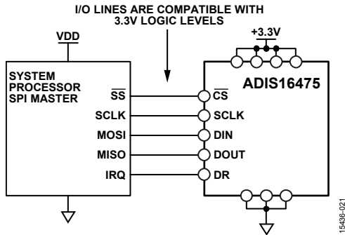
Figure 19. Electrical Connection Diagram
