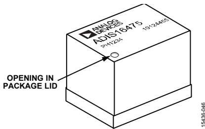
Figure 44. Pressure Relief Hole
