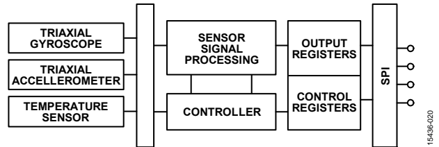
Figure 18. Basic Operation of the ADIS16475
