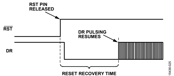
Figure 23. Data Ready Response During Reset ( \overline{RST} = 0 ) Recovery
